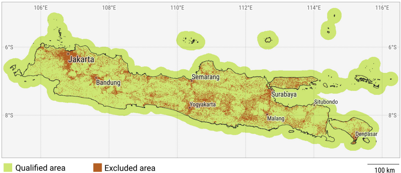
Figure 7 - Localization of the urban areas based on quantification of built-up index, derived from GHS dataset (first); Qualified and excluded areas based on the specified criteria (second)
