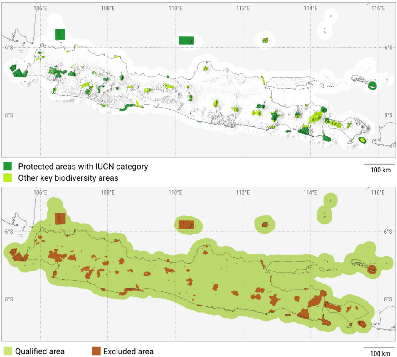
Figure 12 – Protected areas and key biodiversity areas (top); Qualified and excluded areas based on the specified criteria (bottom)
