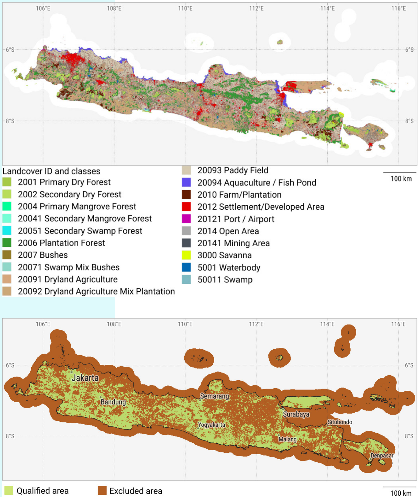
Figure 6 – Land cover classes, based on PL dataset (top); Qualified and excluded areas based on the specified criteria (bottom)
