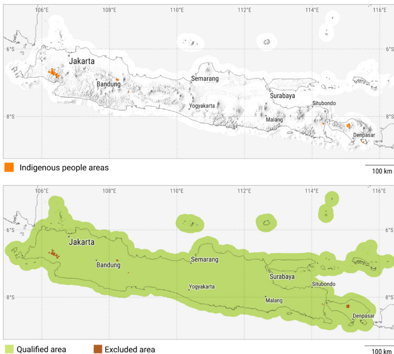
Figure 13 -Location of indigenous people areas (top); Qualified and excluded areas based on the specified criteria (bottom)
