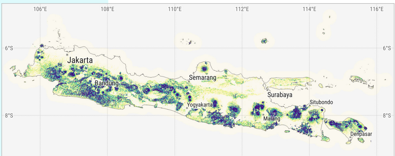
Terrain slope, calculated from SRTM v4.1 terrain data
