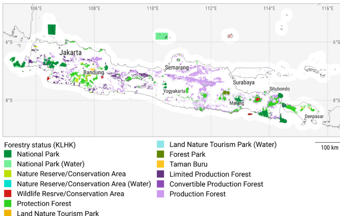
Figure 8 – Qualified and excluded areas based on the specified criteria (first); Forestry status and areas (second);
