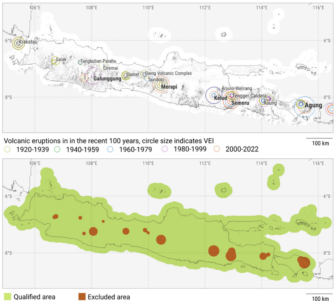
Figure 11 - Volcanic activity in the recent 100 years, based on Global Volcanism Program (top); Qualified and excluded areas based on the specified criteria (bottom)
