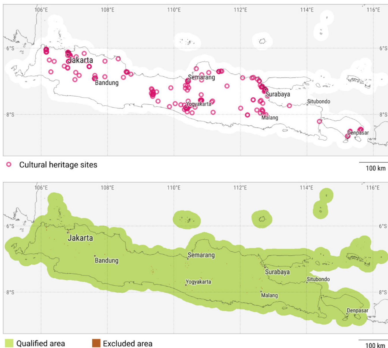
Figure 14 – Location of cultural heritage sites (top); Qualified and excluded areas based on specified criteria based on the specified criteria (bottom)
