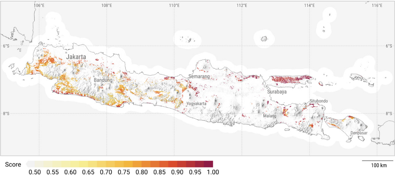
Figure 23 – Geospatial analysis result
