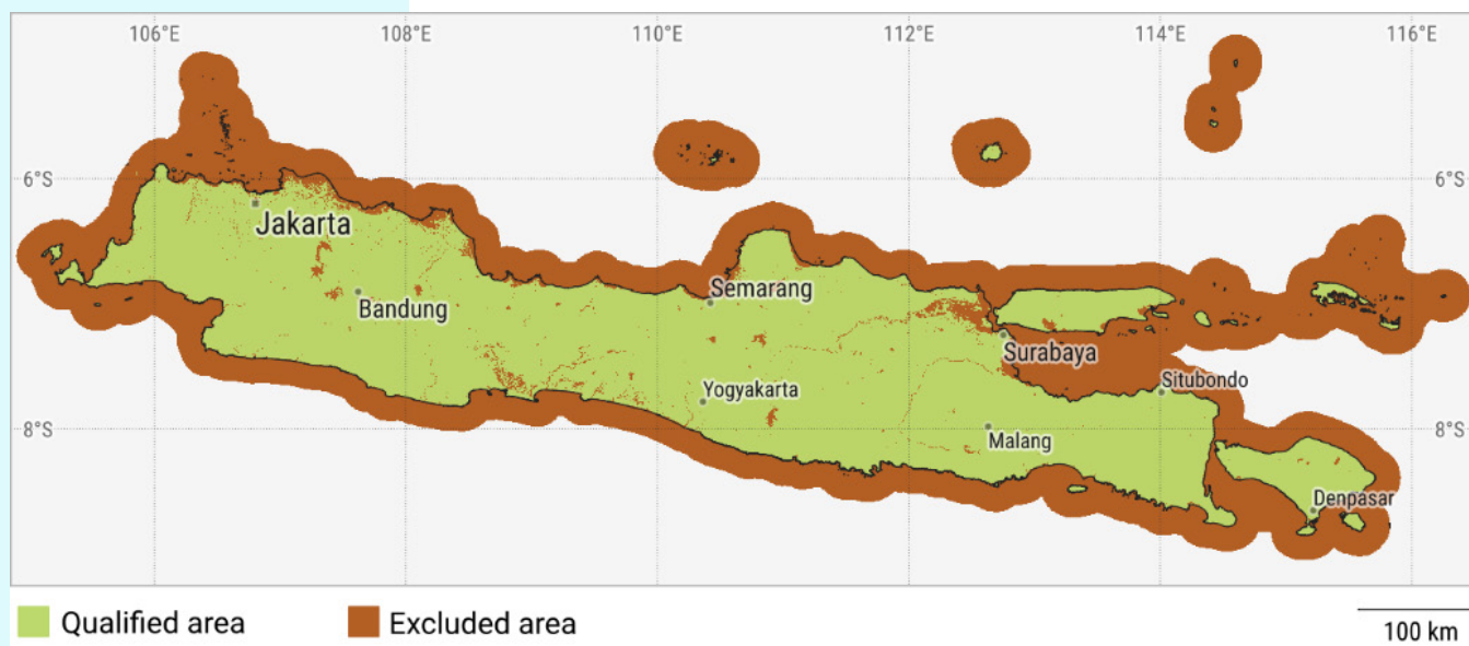
Figure 5 - Occurrence of surface water based on GSW (global surface water) dataset (top); Qualified and excluded areas based on the specified criteria (bottom)
