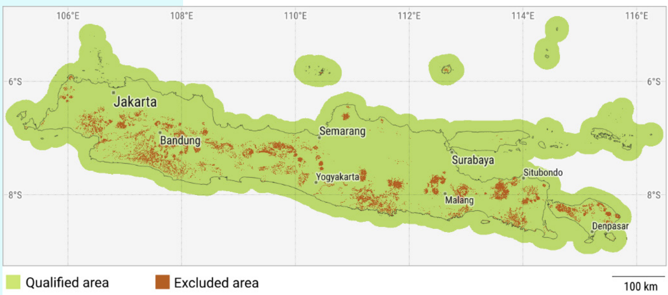
Figure 10 – Terrain slope, calculated from SRTM v4.1 terrain data (top); Qualified and excluded areas based on the specified criteria (bottom)
