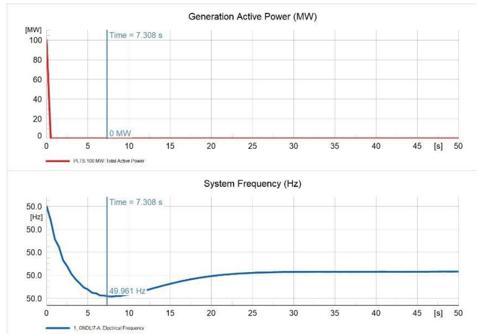
Figure 32 – System frequency simulation
