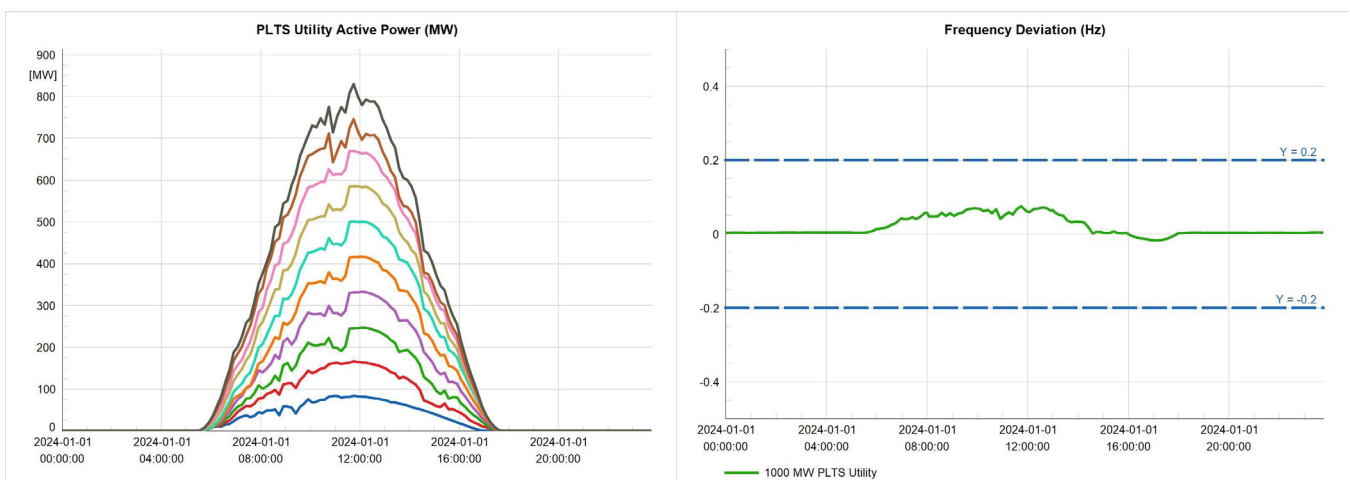
Figure 31 –Utility active power and frequency deviation of 10 PV sites
