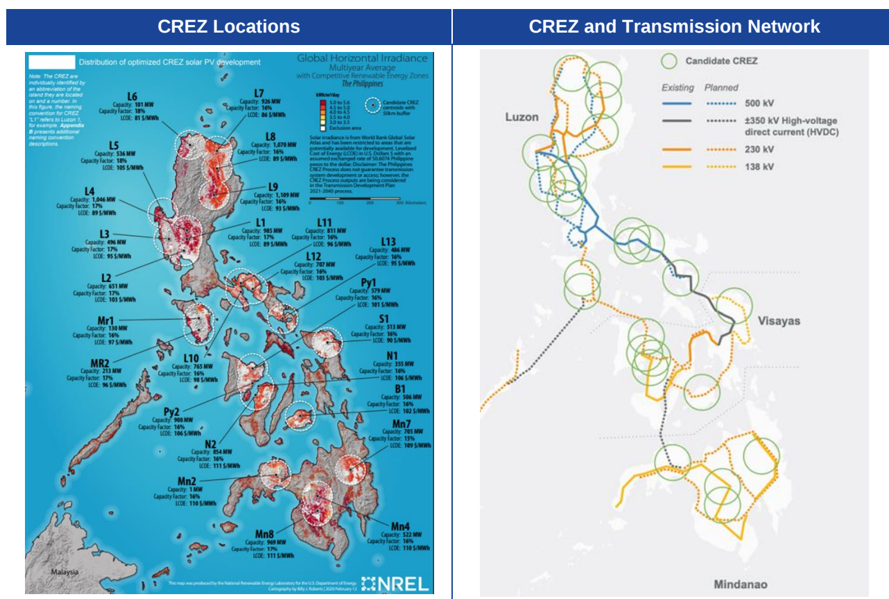
Figure 1. CREZ locations and Transmission Network Proximity
